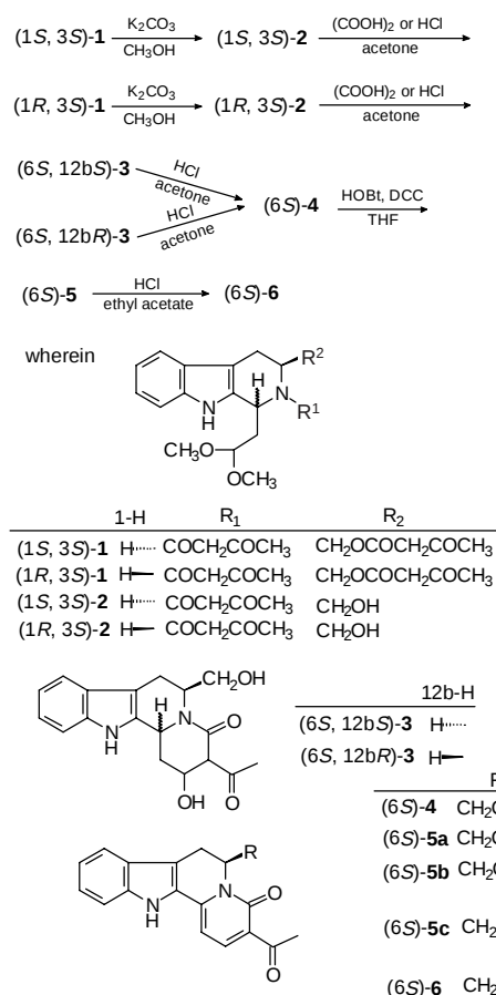
Scheme 1 Synthesis of 6-amino acid ester of (6 S )-3-acetyl-4,6,7,12-tetrahydro-4-oxoindolo[2,3- a ]quinolizine, 5 and 6 from (1 S , 3 S )- 1 and (1 R , 3 S )- 1 by saponification, cyclization, dehydrogenation, dehydration, esterification and deprotection.
